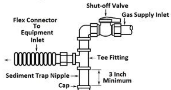
Proper Sediment Trap Installation
