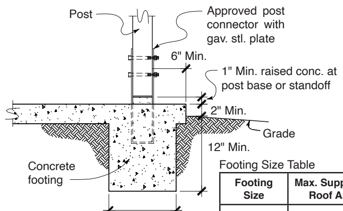
DETAIL D
